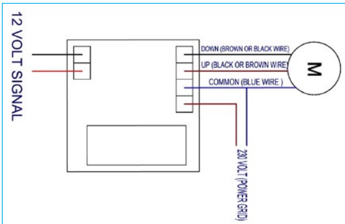
WIRING DIAGRAM
